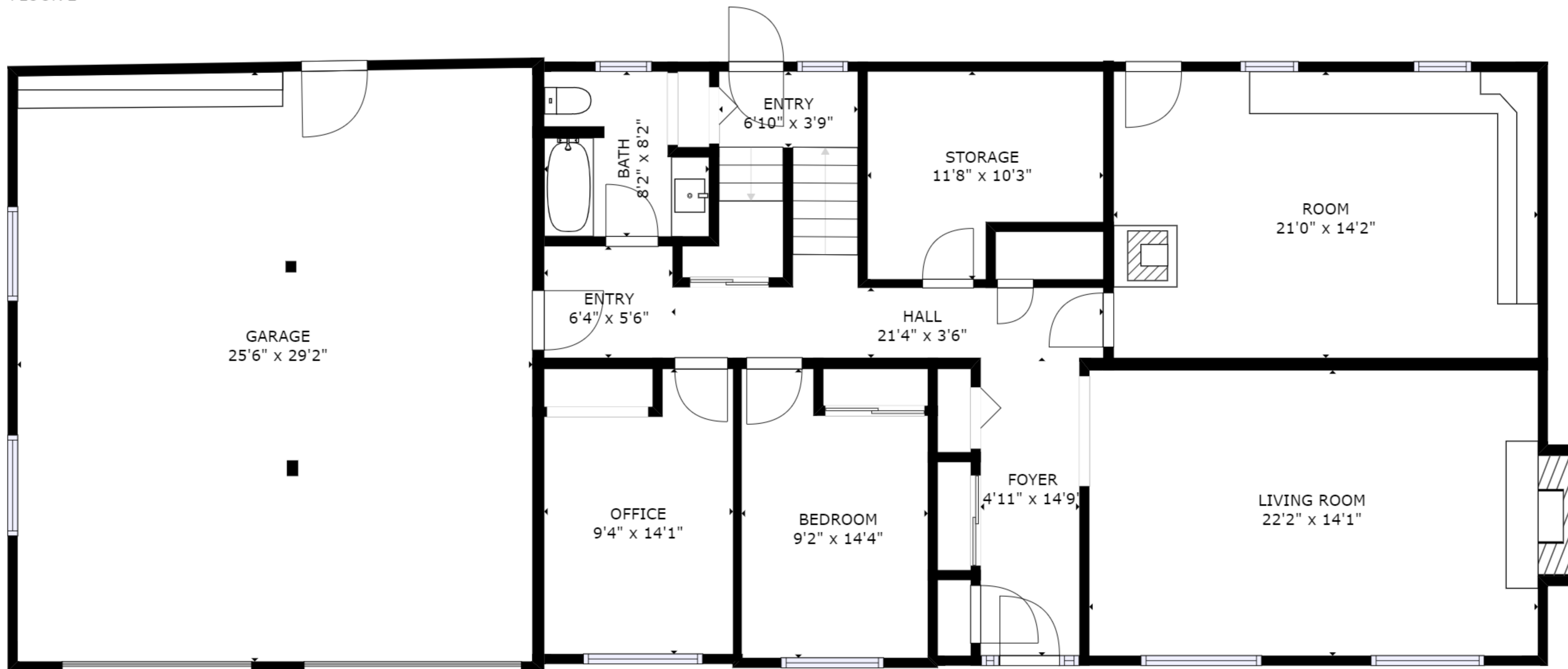
FLOOR 1
