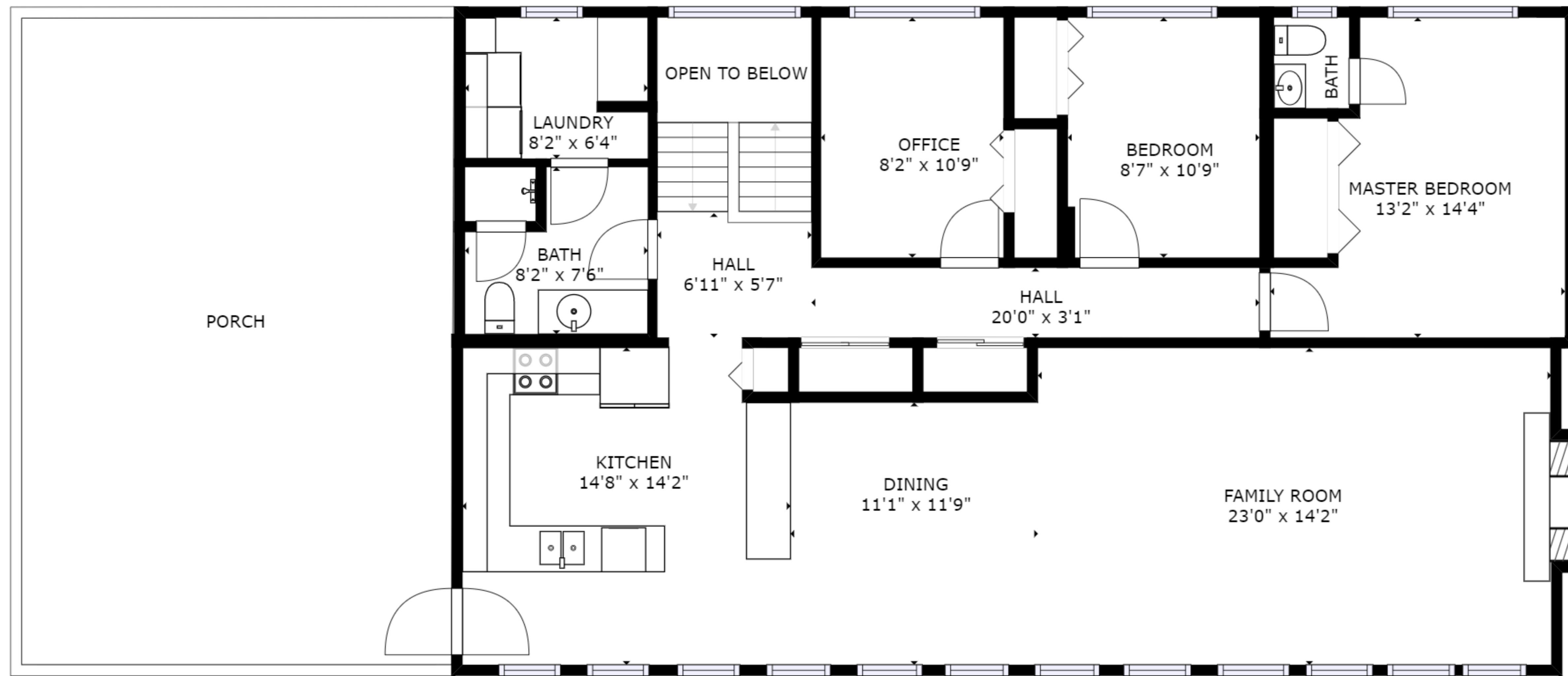
FLOOR 2
